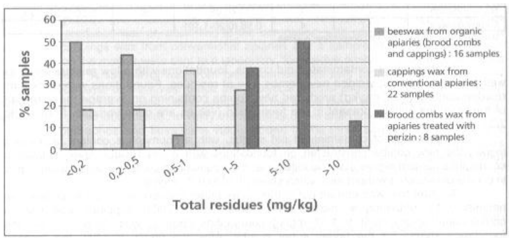
Fig. 1 – Total residues (mg/kg) in wax samples of different origin
